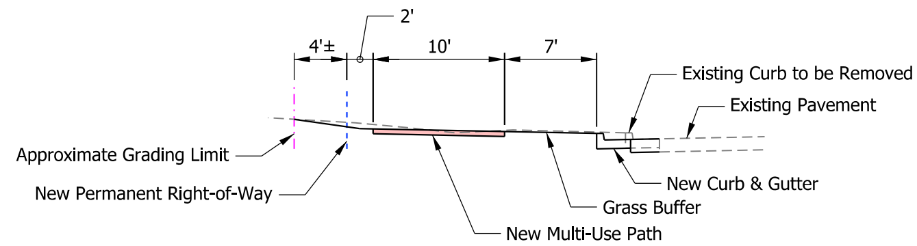
Typical Section - New Multi-Use Path (not to scale)
